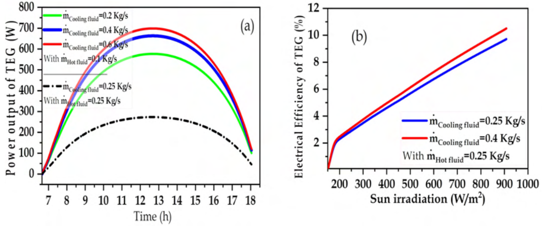
Figure 2: TEG power output (a) and electrical efficiency (b) at various cooling fluid mass flow rate during the day.
