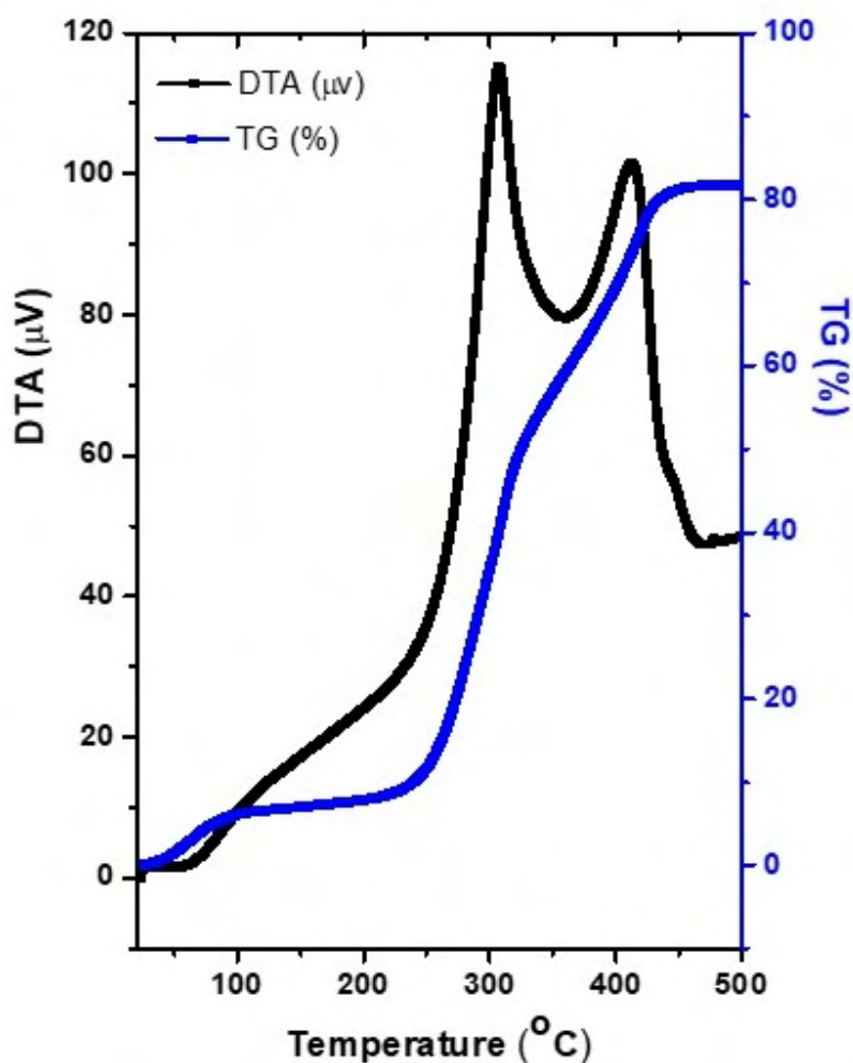
Figure 2: TG and DTA curves of RH.
