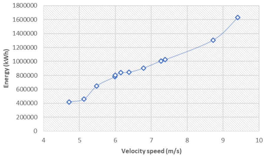
Figure 3: Change of monthly energy production depending on wind speed.
