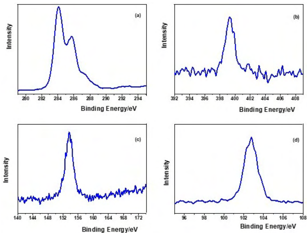
Figure 5: XPS spectra of RH sample (a) C1s, (b) N1s, (c) S2p (d) Si2p.
